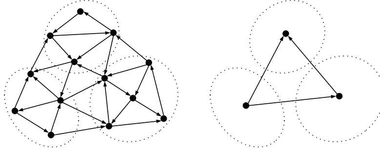
Figure 5.5: Examples of node and edge aggregates produced by the cSA method. In this case, three coarse edges are induced by the nodal aggregation.
