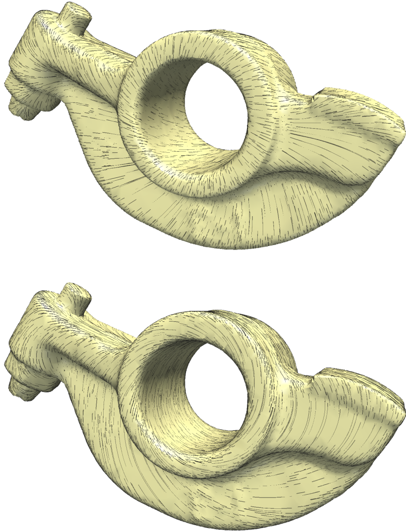
Figure 7.1: The two harmonic 1-forms of a rocker arm surface mesh.
